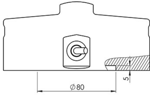
CM (CM-Ex) Capacity 30 to 50 ton
