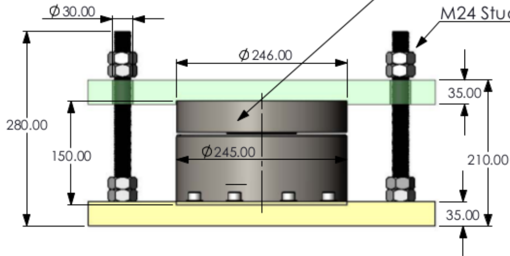
Eilersen GDS/DH 100 Ton Load Cell
